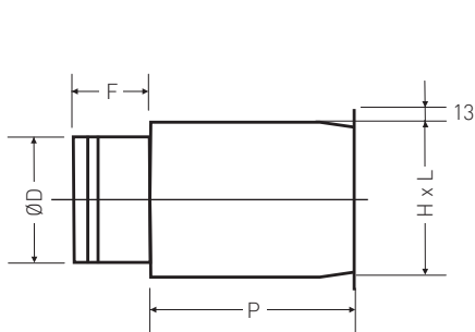
PBOS-PBOI Plenum with rear connection
