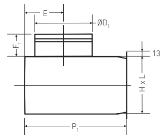
PBVS-PBVI Plenum with side connection
