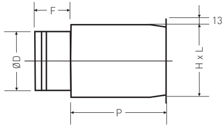
PBOS-PB0I Plenum with rear connection
